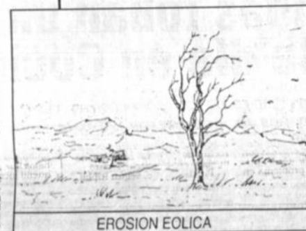
EROSION EOLICA
