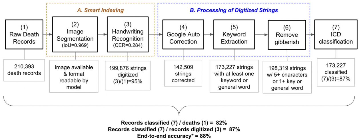
Fig. 3. Summary of Processing Pipeline and Performance Metrics.
