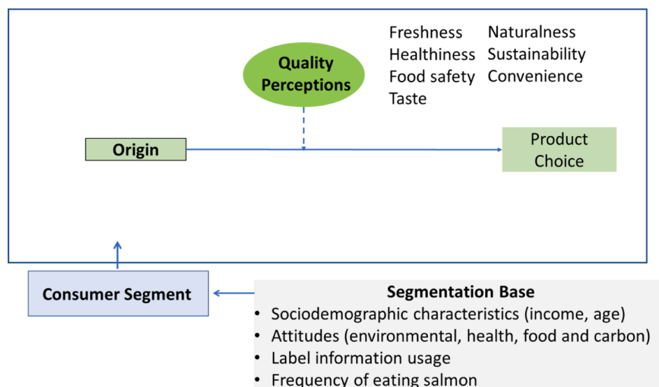
Fig. 1. Conceptual Framework.
