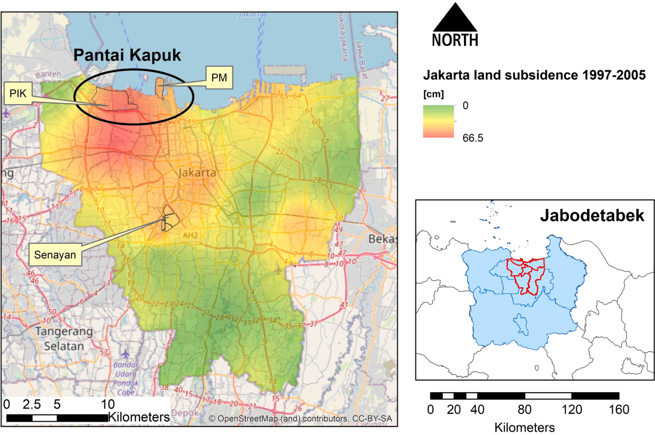
Fig. 1. Jakarta's land subsidence (1997–2005).
