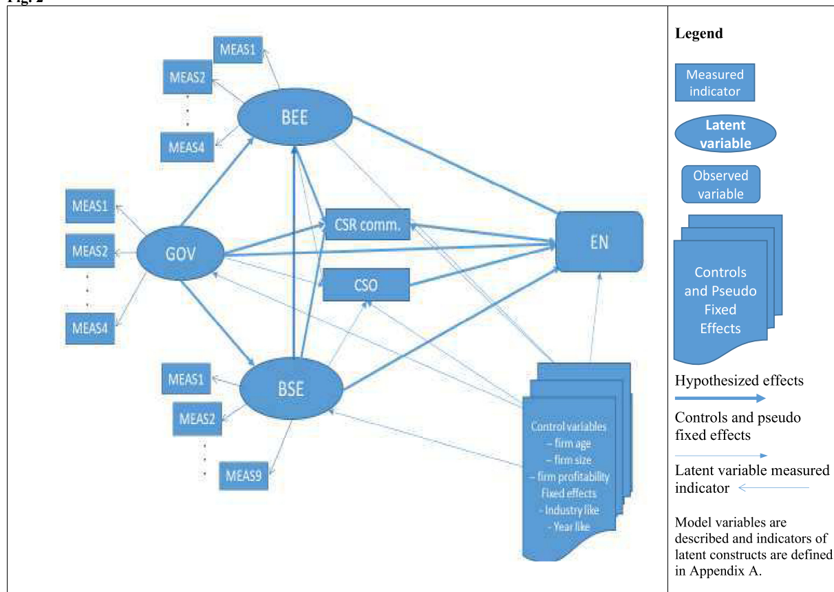
Fig. 2. Mixed SEM Measurement Model Estimated.
