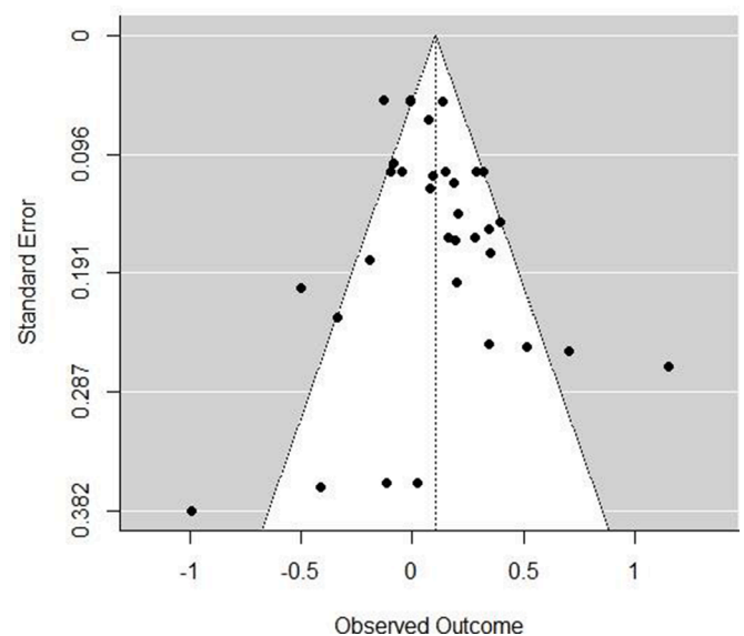
Fig. 3. Funnel plot.
