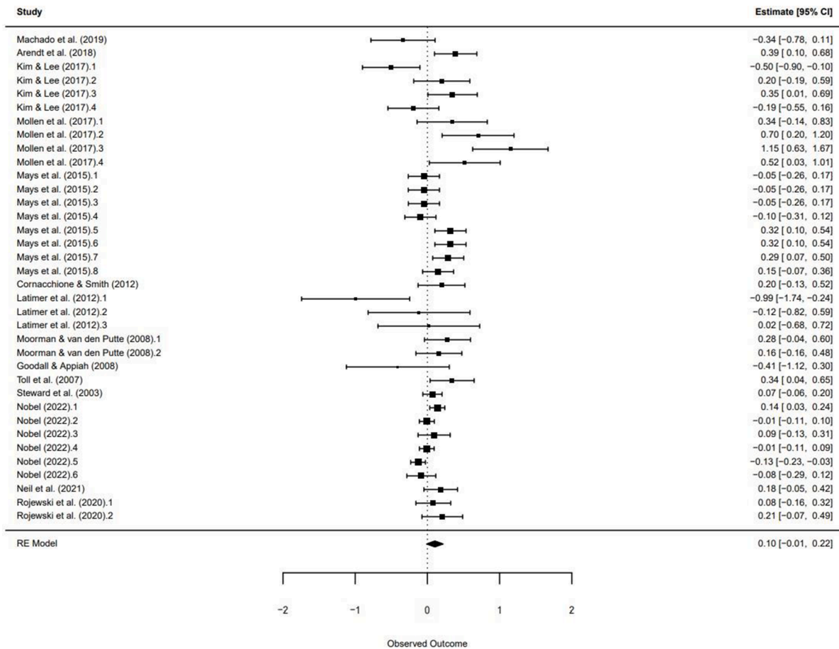
Fig. 1. Forest plot.
