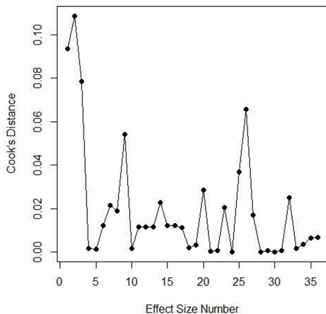
Fig. 2. Cook's distance.
