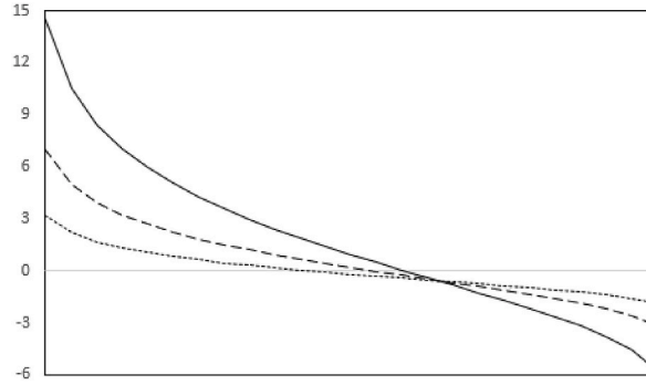
Fig. 1. Plot of E[\Delta\tilde{u}_i(x_i) - \tilde{u}_0] with m = 25 , a_0 = a_i = 0 , and \beta = 1 (dotted curve), \beta = 2 (dashed curve), \beta = 4 (solid curve). The x-axis ranges from x_i = 1 to x_i = 25 . Expressions for E[\Delta\tilde{u}_i(x_i) - \tilde{u}_0] appear in Lemma 6.
