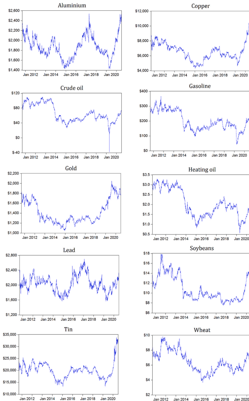
Fig. 1. Time-series graph of raw U.S. dollar commodity prices.
