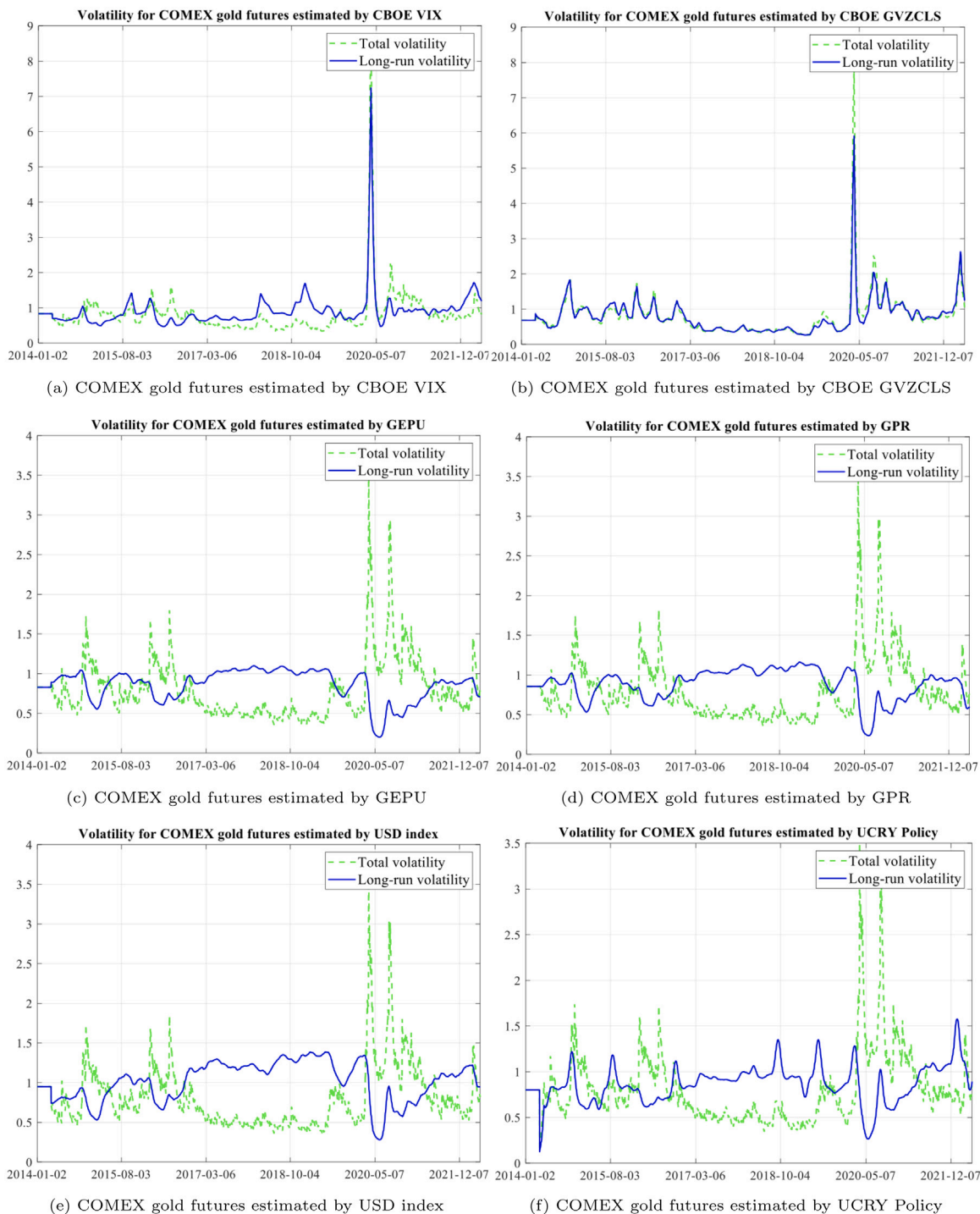
Fig. 2. Estimated total and long-term volatilities of COMEX gold futures by various monthly uncertainty indices. Notes: This plot shows the estimated total daily volatility and long-term volatility of GARCH-MIDAS. The green dashed line indicates the COMEX Gold Futures total daily volatility, and the blue line means the COMEX Gold Futures long-term volatility determined by CBOE VIX, CBOE GVZCLS, GEPU, GPR, USD index and UCRY Policy, these uncertainty indices. The COMEX Gold Futures is in the high-frequency daily data, and the uncertainty indices are all in the low-frequency monthly data. The sample is from 02/Jan/2014 to 13/May/2022. (For interpretation of the references to colour in this figure legend, the reader is referred to the web version of this article.)
