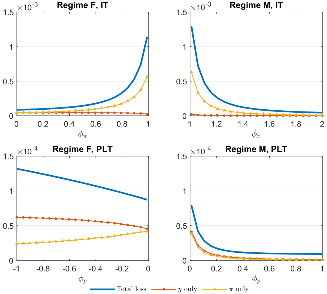
Fig. 2. Loss function after a demand shock.
