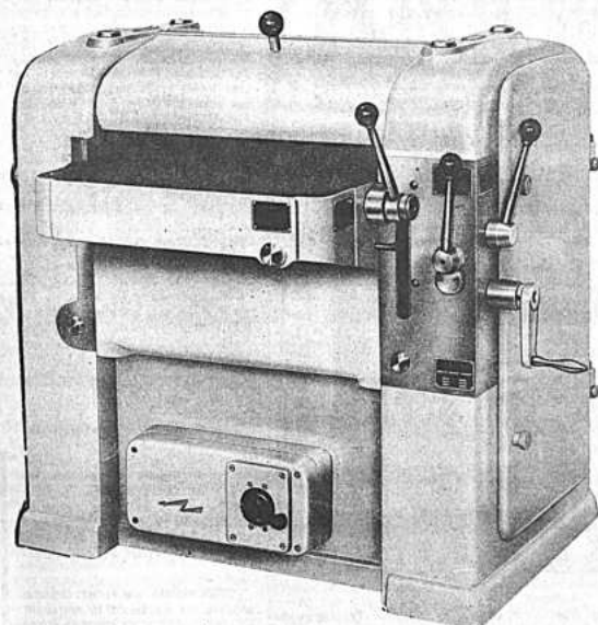
Regruessadora - T40
