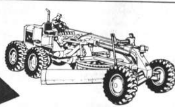
ALLIS-CHALMERS M-100B 167 hp • Weight approx. 27,150 lbs. equipped as shown
